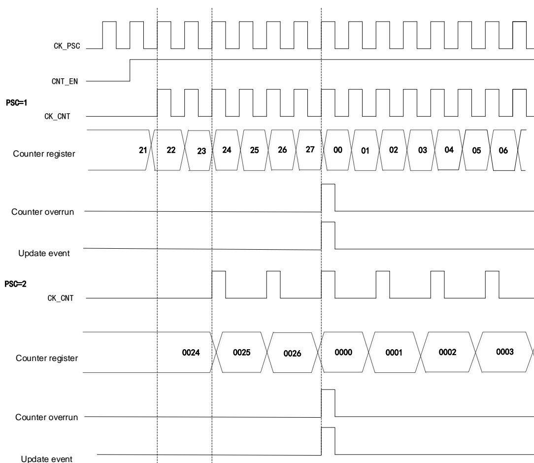
Figure 67 Timing Diagram when Division Factor is 1 or 2 in Count-up Mode
