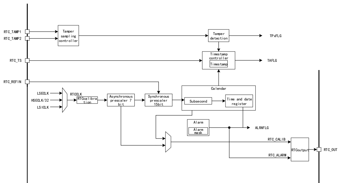
Figure 83 APM32F030x6x8 RTC Structure Block Diagram
