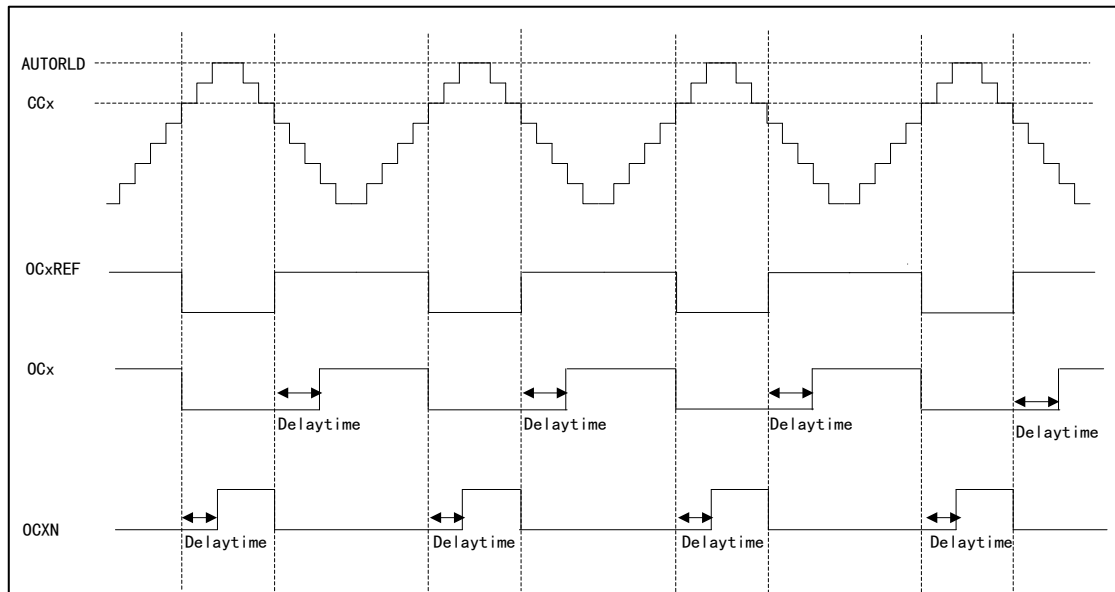
Figure 38 Complementary Output of Insertion with Dead-time
