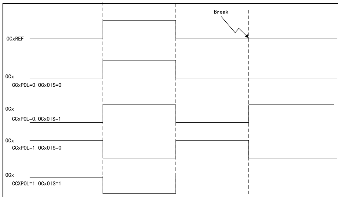
Figure 74 Breaking Event Timing Diagram
