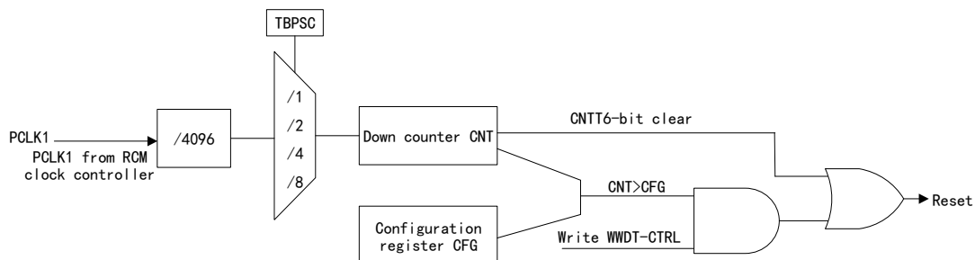
Figure 81 Window Watchdog Structure Block Diagram
