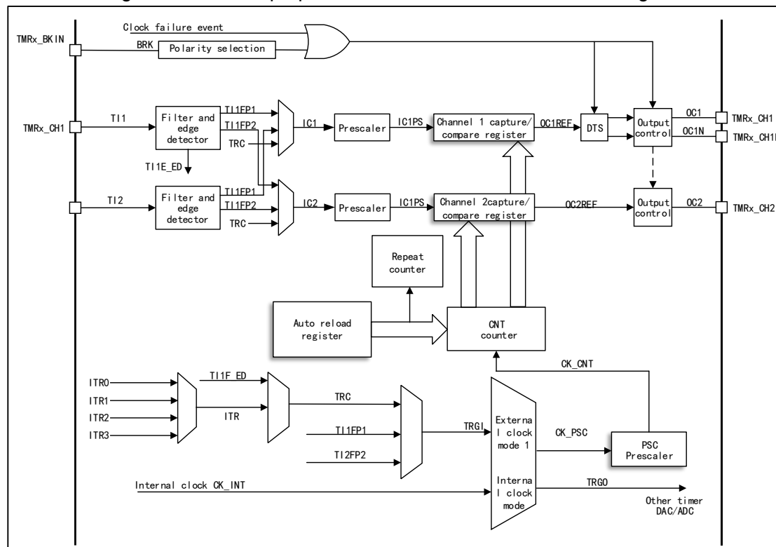
Figure 65 General-purpose Timer TMR15 Structure Block Diagram
