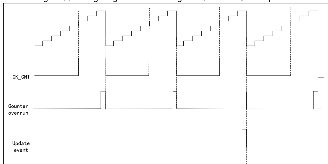
Figure 68 Timing Diagram when Setting REPCNT=2 in Count-up Mode
