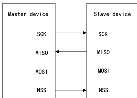
Figure 100 Connection in Simplex Mode (the master is used for receiving, while the slave is used for transmitting)
