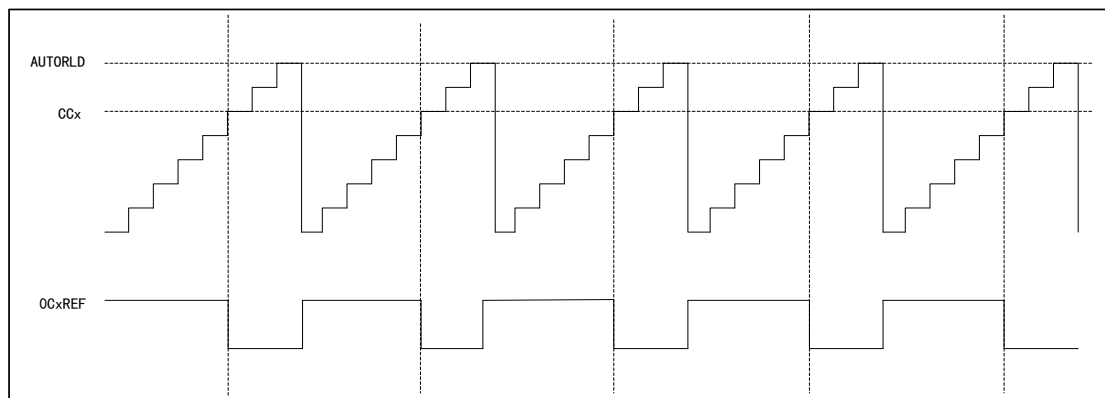
Figure 63 PWM1 Count-up Mode Timing Diagram
