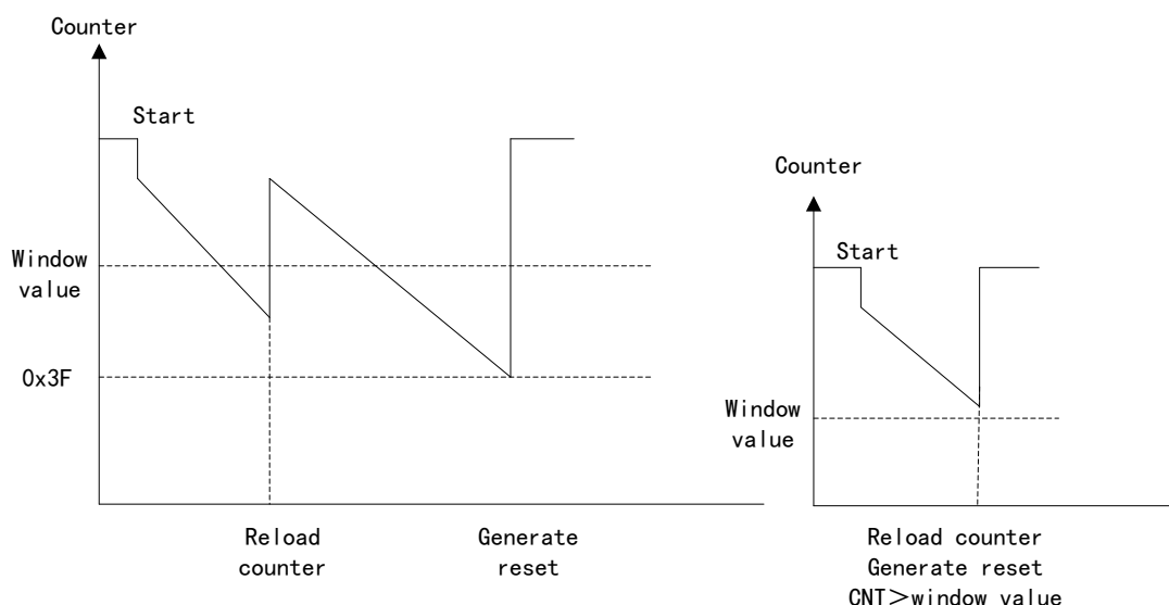
Figure 82 Window Watchdog Timing Diagram
