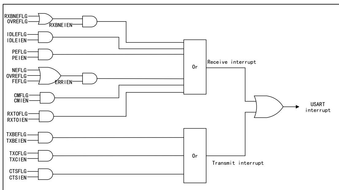
Figure 91 USART Interrupt Mapping
