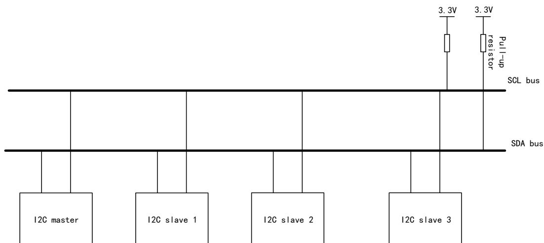
Figure 94 Commonly Used I2C Communication Connection Diagram
