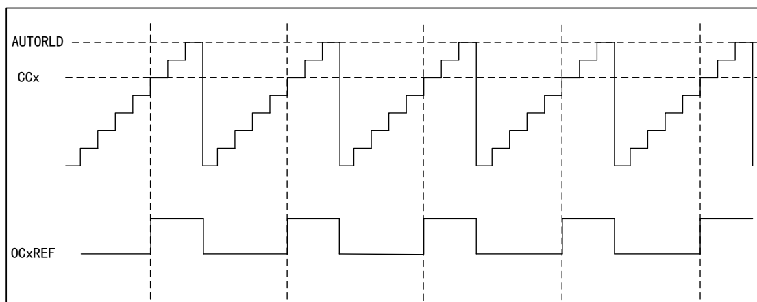
Figure 64 PWM2 Count-up Mode Timing Diagram
