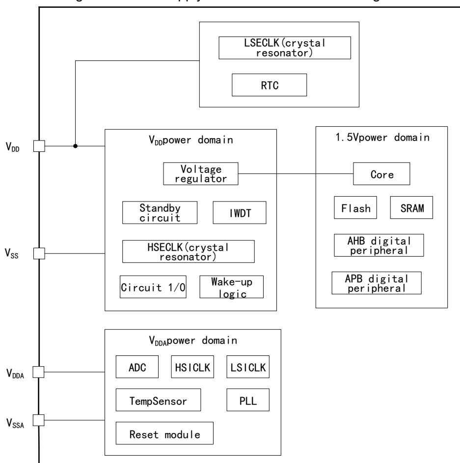
Figure 7 Power Supply Control Structure Block Diagram
