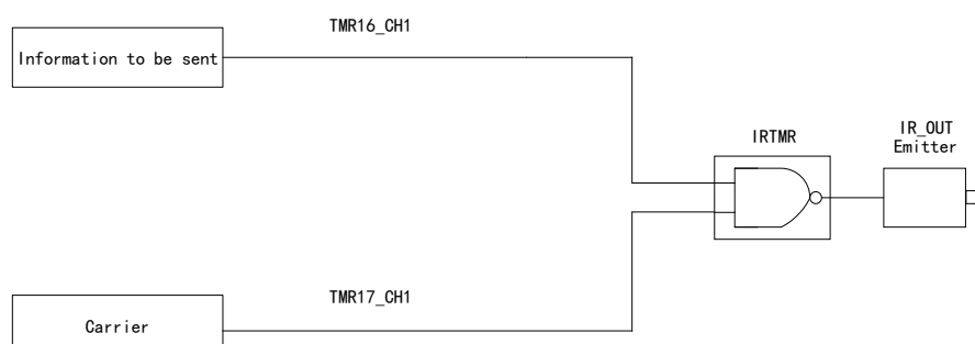
Figure 79 IRTMR Structure Block Diagram
