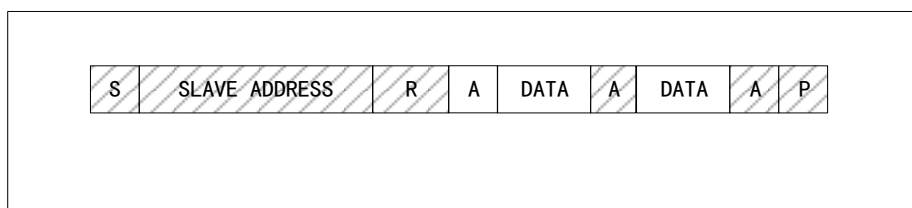
Figure 96 Master Reads Data from Slave
