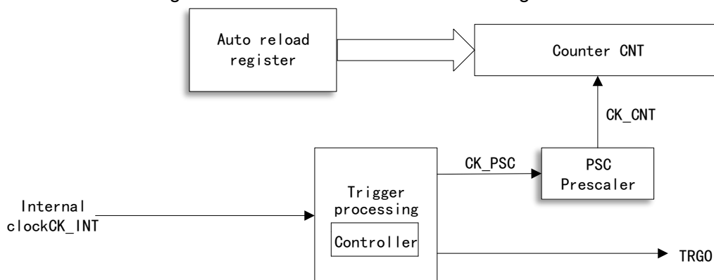
Figure 77 Basic Timer Structure Block Diagram
