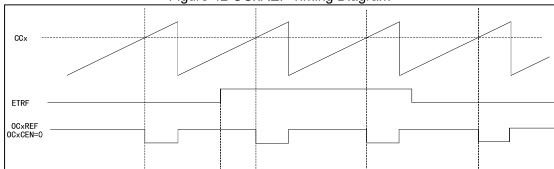
Figure 42 OCxREF Timing Diagram
