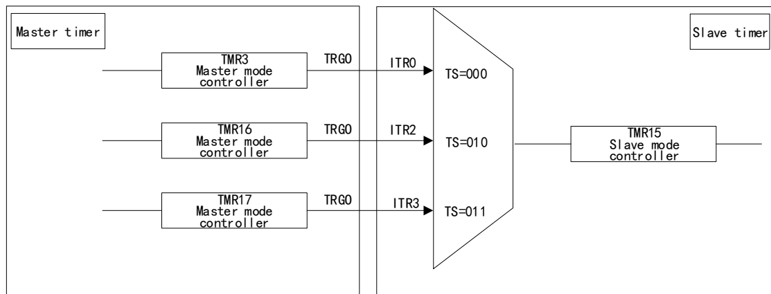
Figure 76 Interconnection of TMR15 and Other Timers
