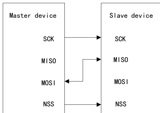
Figure 99 Connection in Half Duplex Mode
