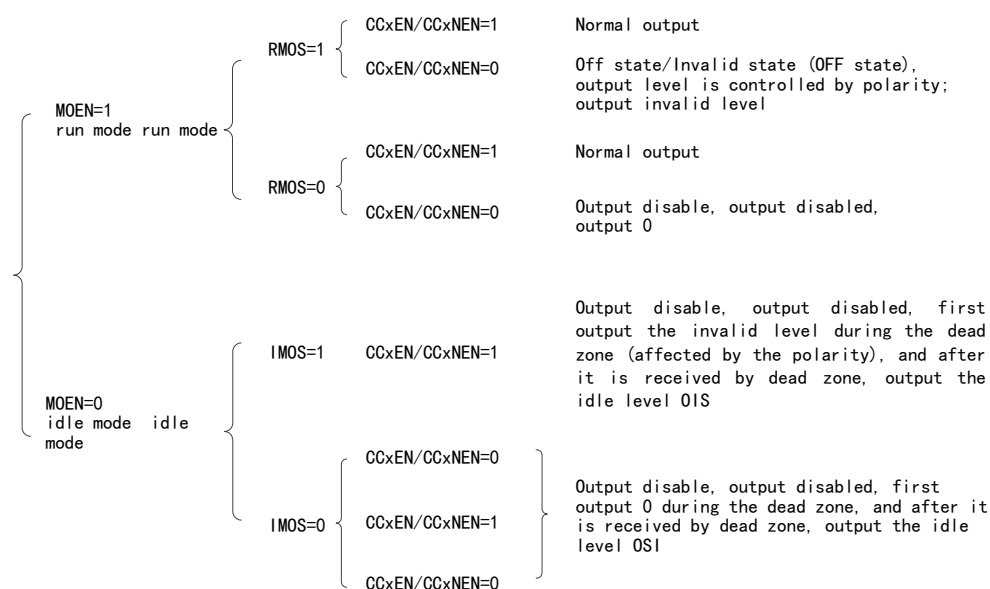
Figure 73 Register Structural Relationship Affecting Output Waveform
