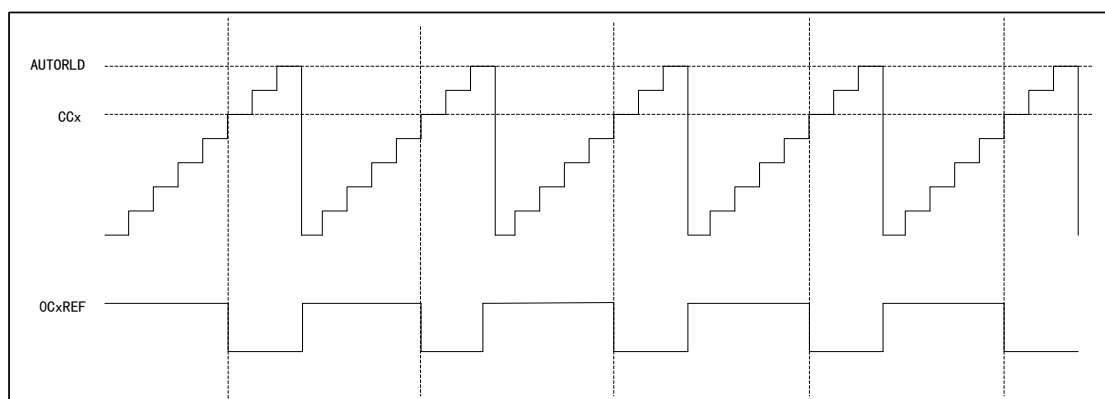
Figure 69 PWM1 Count-up Mode Timing Diagram
