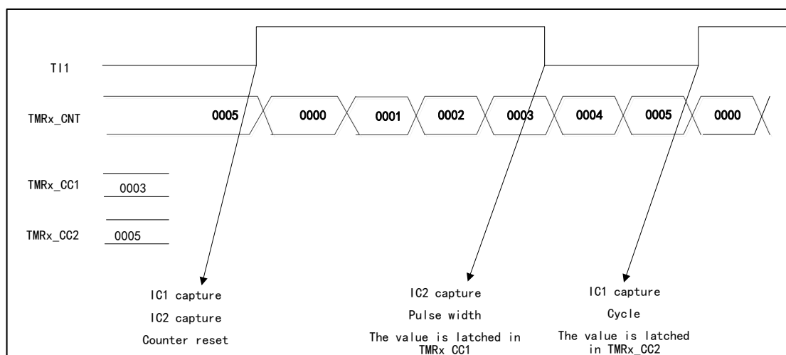
Figure 54 Timing Diagram in PWM Input Mode
