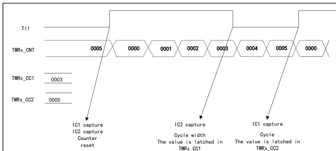
Figure 71 Timing Diagram in PWM Input Mode
