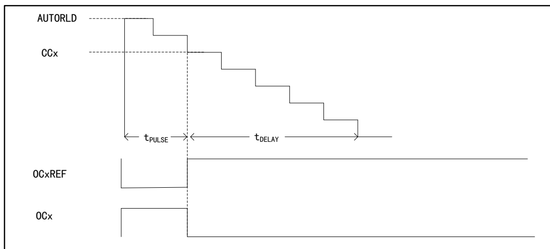
Figure 72 Timing Diagram in Single-pulse Mode
