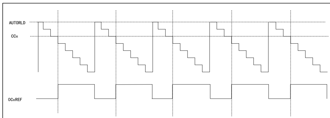
Figure 29 PWM1 Count-down Mode Timing Diagram
