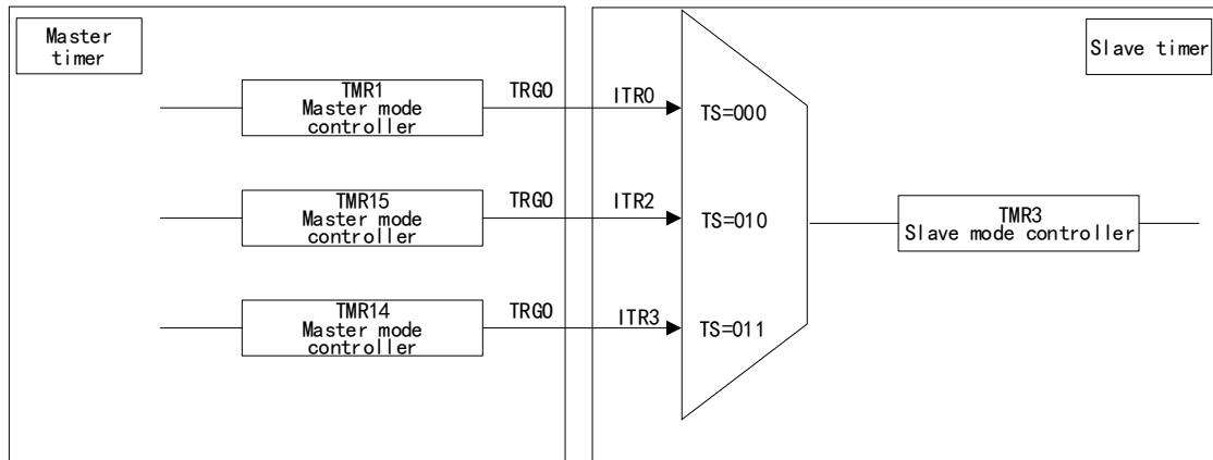
Figure 58 Interconnection of TMR3 and Other Timers
