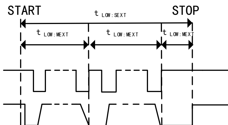
Figure 97 t_{\text{LOW:SEXT}} and t_{\text{LOW:MEXT}} Time
