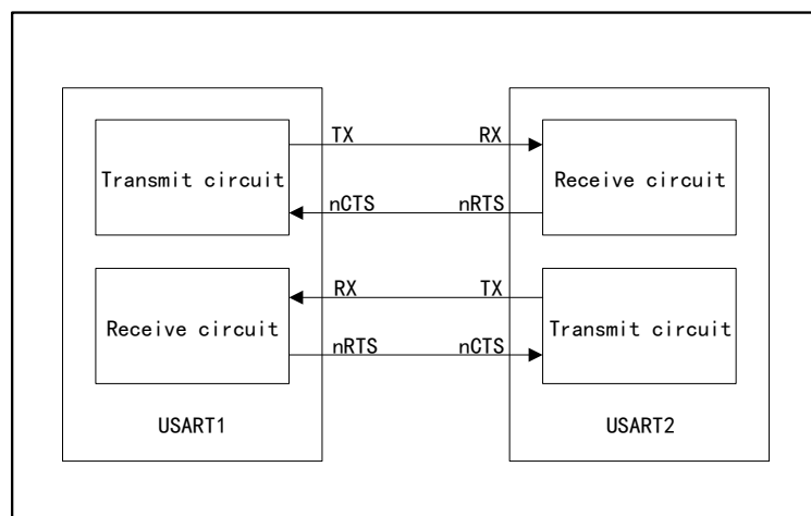
Figure 90 Hardware Flow Control between Two USARTs
