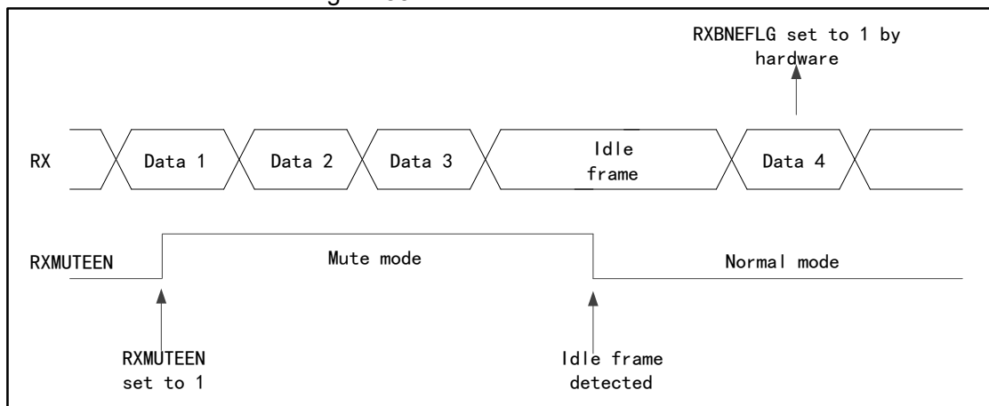
Figure 85 Idle Bus Exit Mute Mode
