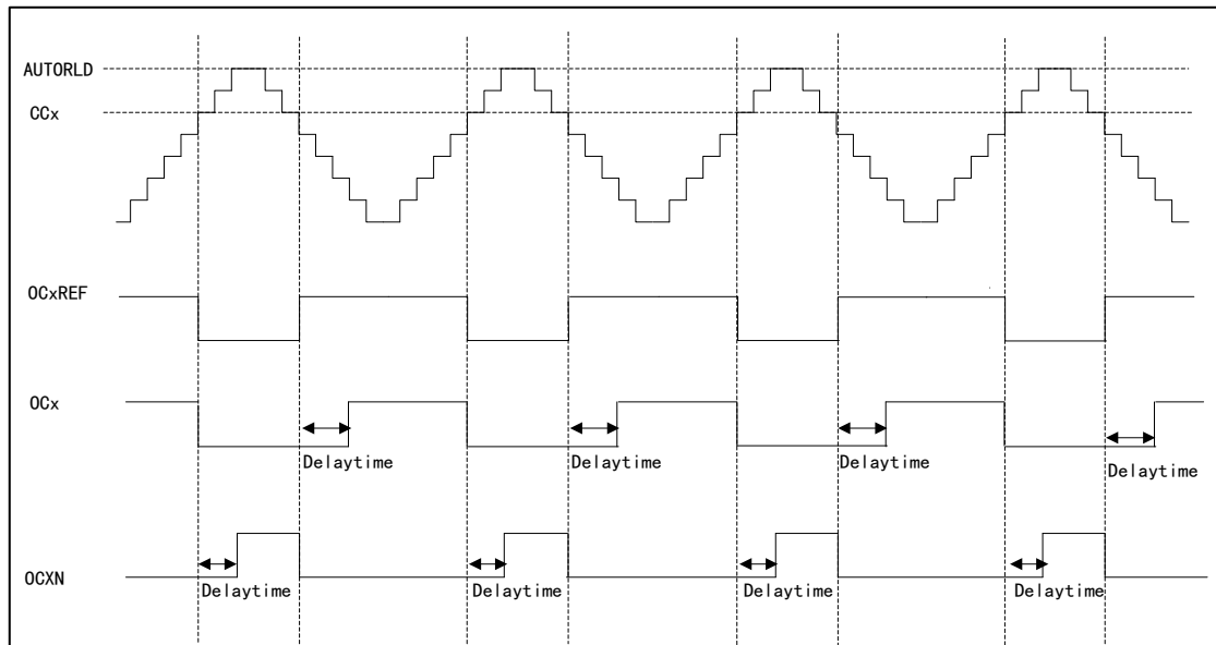
Figure 75 Complementary Output of Insertion with Dead-time
