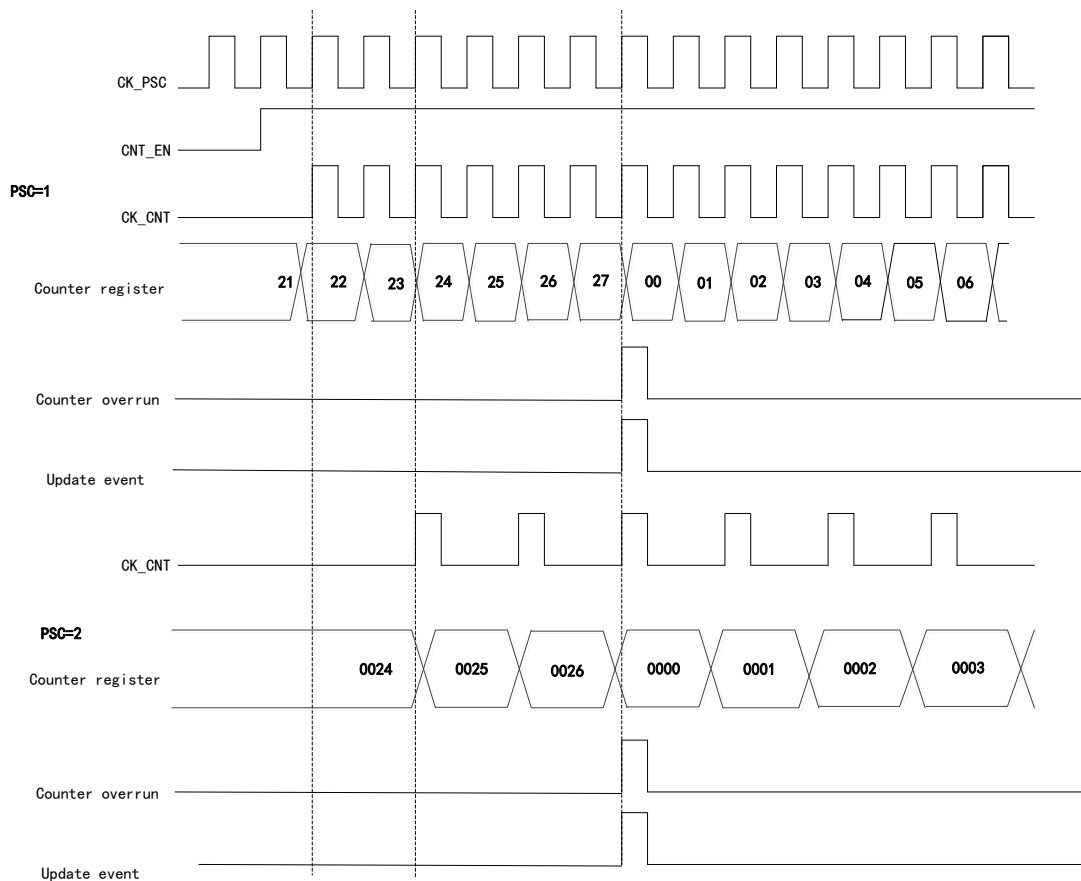
Figure 78 Counter Timing Diagram, the internal clock division factor is 1 or 2
