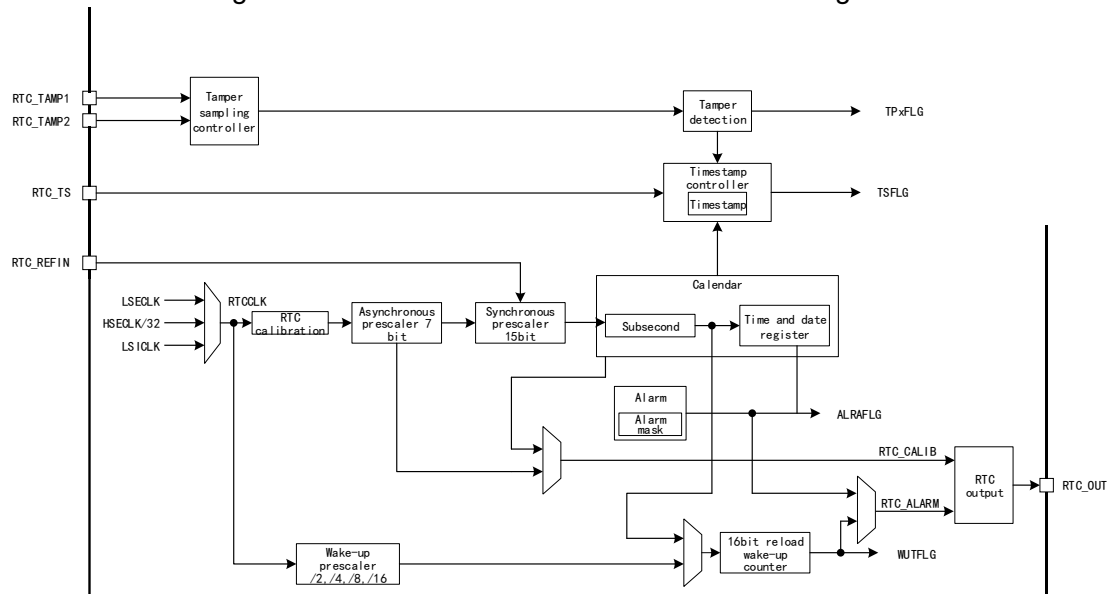
Figure 84 APM32F030xC RTC Structure Block Diagram
