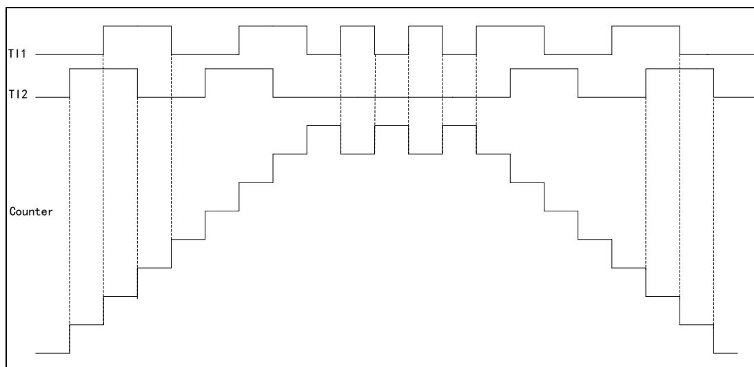
Figure 56 Counter Operation Example in Encoder Mode
