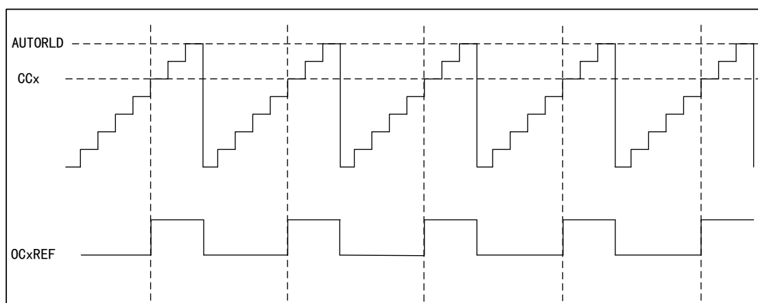
Figure 70 PWM2 Count-up Mode Timing Diagram
