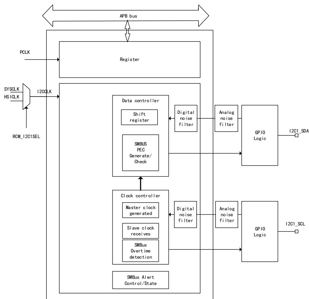
Figure 92 I2C1 Functional Structure Diagram
