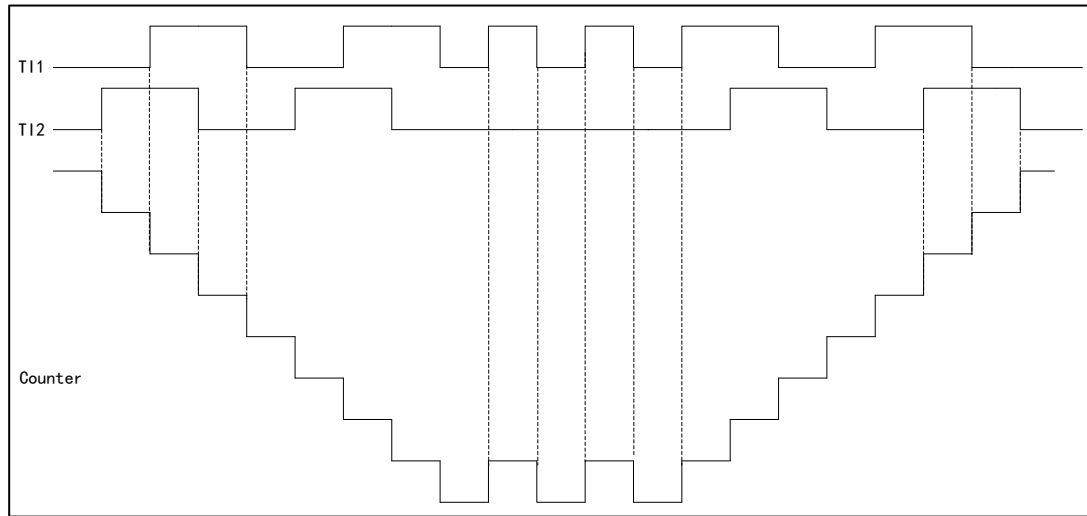
Figure 57 Example of Encoder Interface Mode of TI1FP1 Reversed Phase
