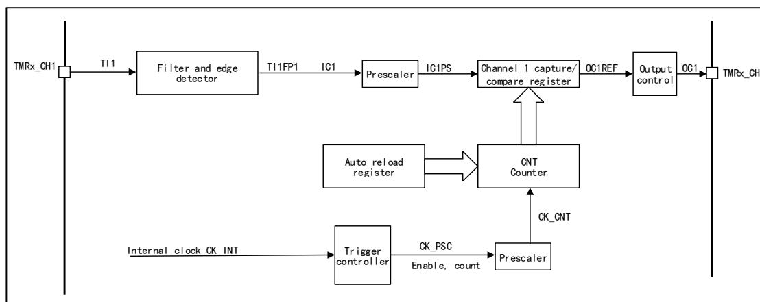
Figure 61 General-purpose Timer TMR14 Structure Block Diagram
