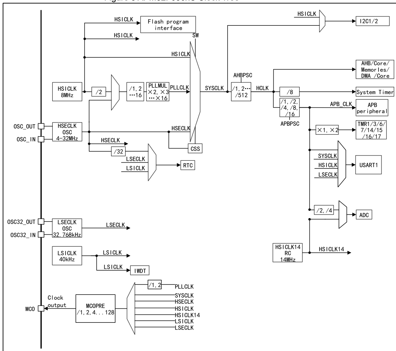
Figure 5 APM32F030xC Clock Tree
