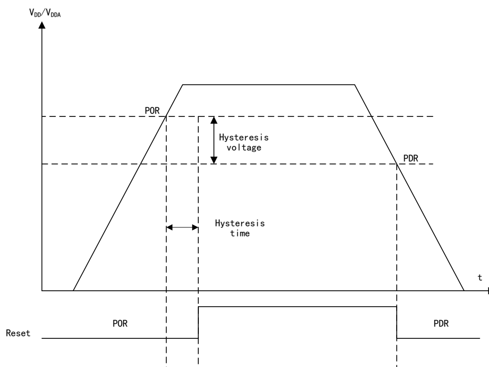
Figure 8 Power-on Reset and Power-down Reset Oscillogram
