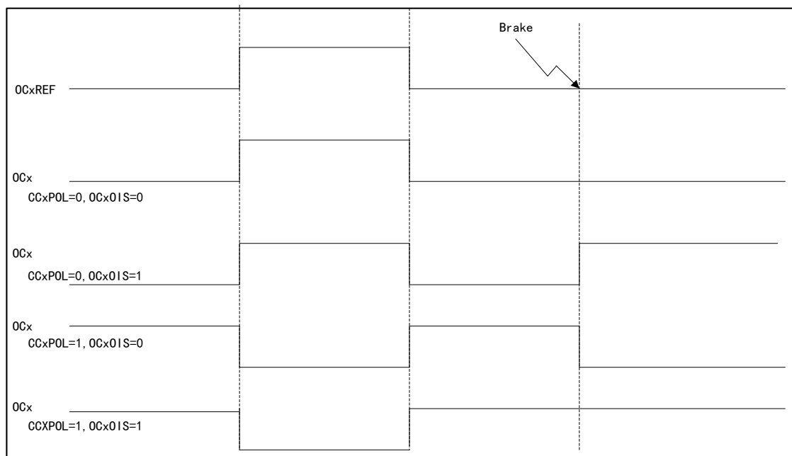
Figure 37 Breaking Event Timing Diagram
