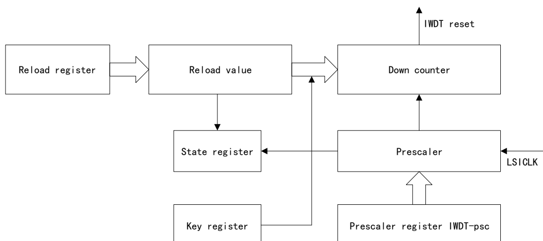
Figure 80 Independent Watchdog Structure Block Diagram
