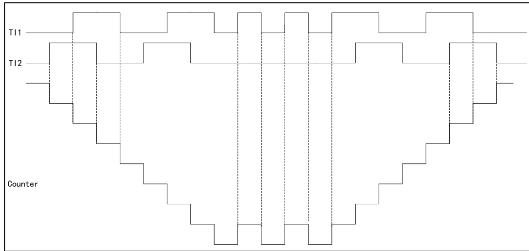
Figure 40 Example of Encoder Interface Mode of TI1FP1 Reversed Phase
