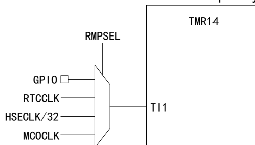
Figure 6 TMR14 Indirect Measurement Clock Frequency Circuit Diagram
