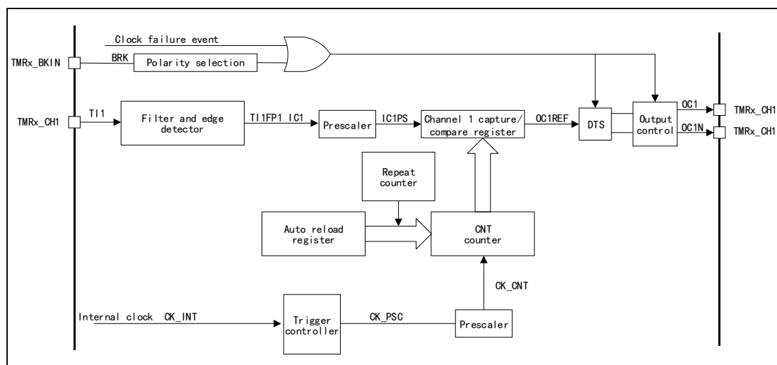
Figure 66 General-purpose Timer TMR16/17 Structure Block Diagram
