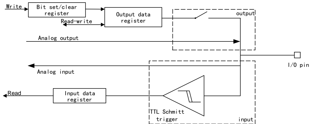
Figure 21 Analog Function I/O Structure
