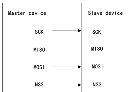
Figure 101 Connection in Simplex Mode (the master only transmits, while the slave receives)
