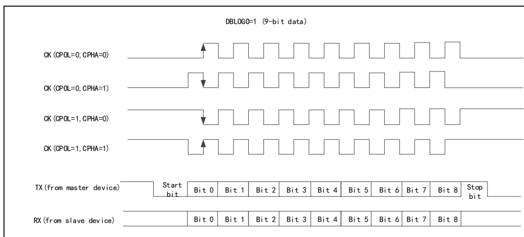
Figure 89 USART Synchronous Transmission Timing Diagram (DBLCFG0=1)
