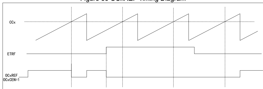
Figure 60 OCxREF Timing Diagram
