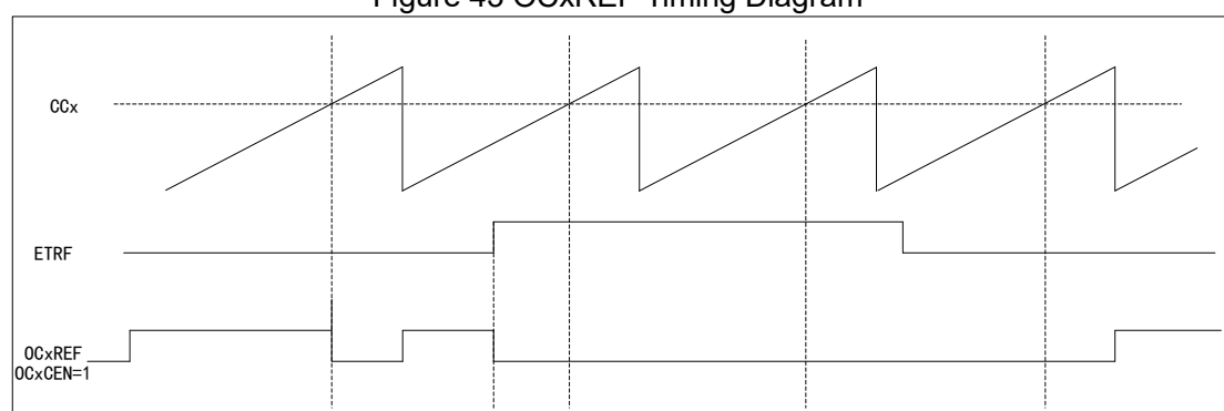
Figure 43 OCxREF Timing Diagram
