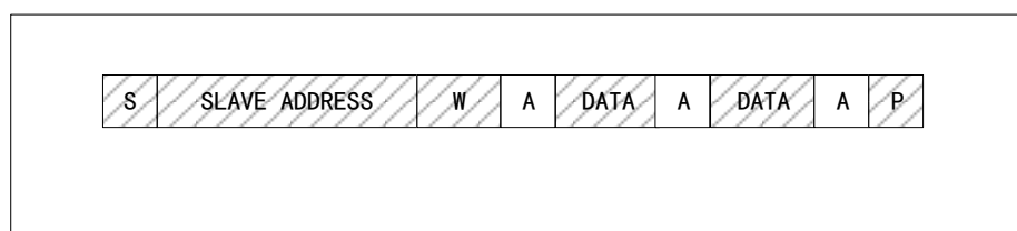
Figure 95 Master Writes Data to Slave
