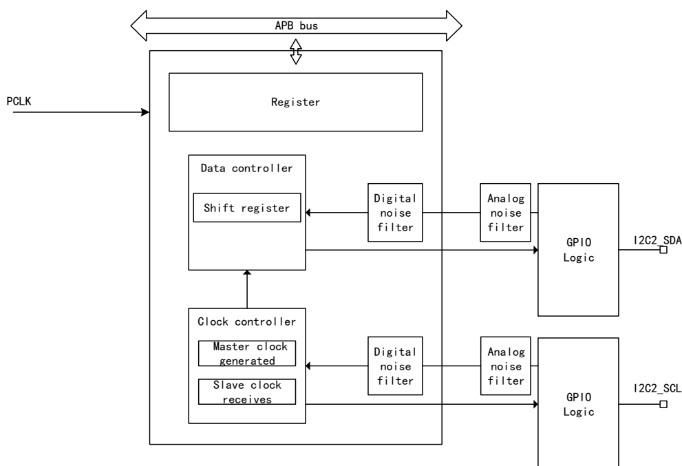
Figure 93 I2C2 Functional Structure Diagram
