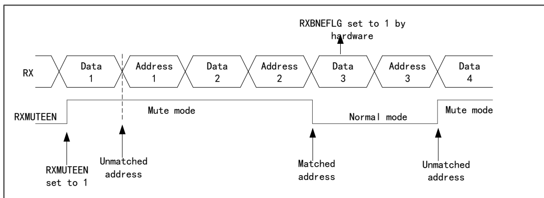
Figure 86 Address Flag Exit Mute Mode
